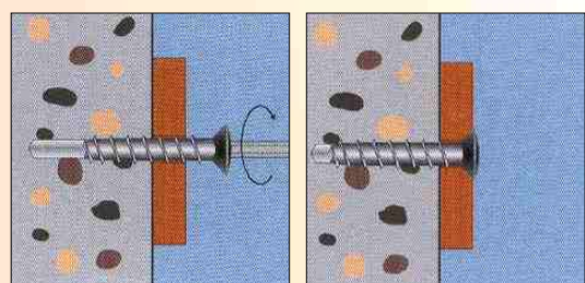
3 - Aparafusar o MULTI-MONTI
